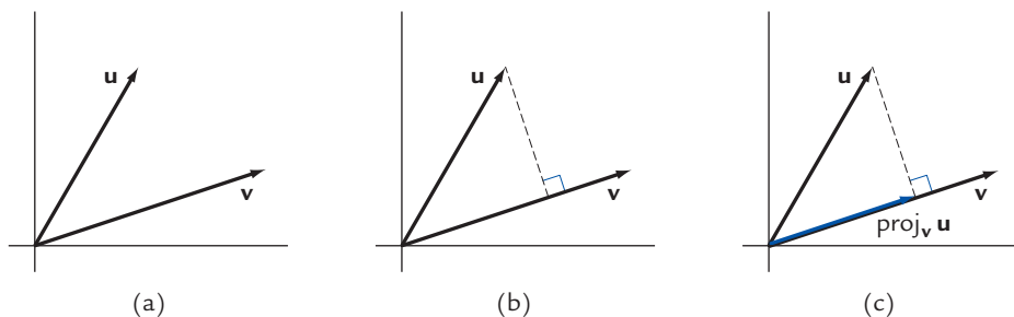
Figure 1 Constructing \text{proj}_{\mathbf{v}} \mathbf{u} in \mathbb{R}^2 .
