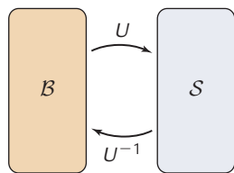
Figure 1 Change of basis between \mathcal{S} and \mathcal{B} .
