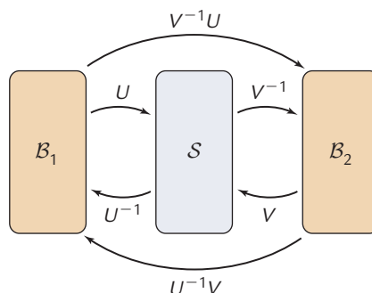
Figure 2 Change of basis between \mathcal{B}_1 and \mathcal{B}_2 .
