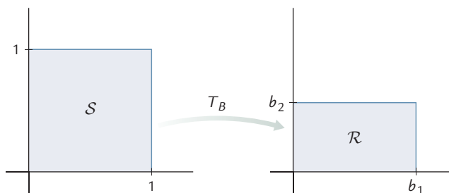
Figure 5 The image of S under T_B is the rectangular region \mathcal{R} .
