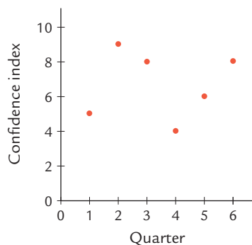
Figure 4 Consumer confidence index data.
