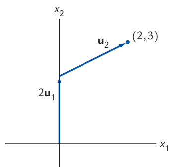
Figure 2 2\mathbf{u}_1 + \mathbf{u}_2 = (2, 3) .
