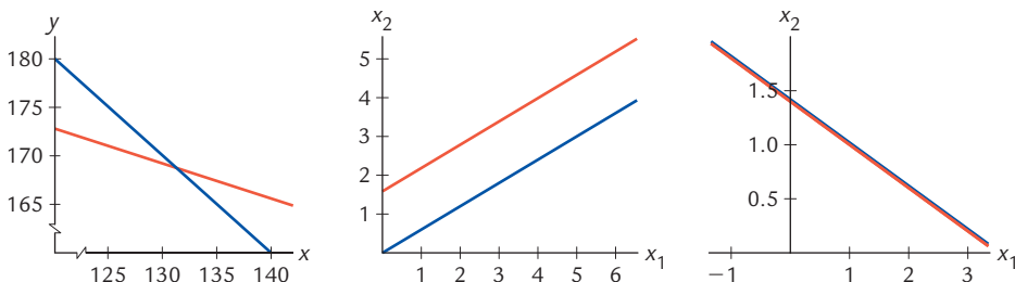
Figure 6 Graphs of equations in Examples 1–3.
