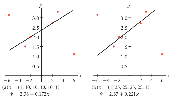
Figure 4 The graphs of weighted least squares regression lines with weights as shown.
