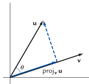
Figure 4 The angle \theta between \mathbf{u} and \mathbf{v} .
