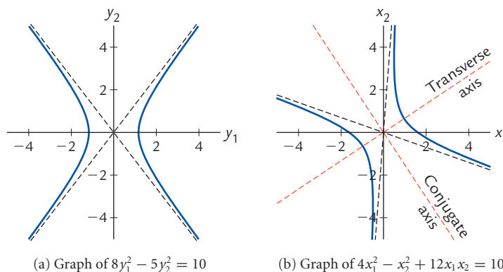
Figure 4 In (a), the graph of 8y_1^2 - 5y_2^2 = 10 , which is in standard position. Rotating this graph to align the axes of symmetry with the eigenvectors of A gives the graph of 4x_1^2 - x_2^2 + 12x_1x_2 = 10 in (b).
