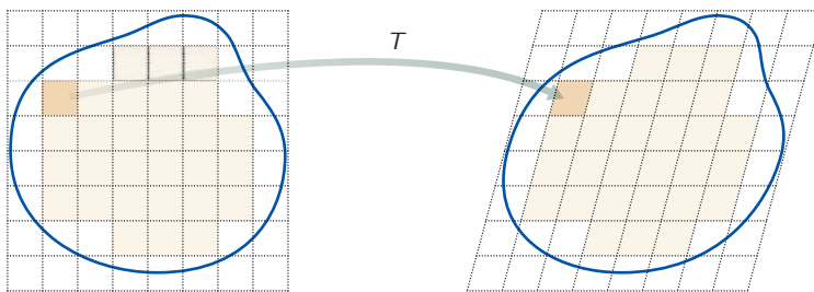
Figure 8 A grid of squares over \mathcal{D} and the corresponding parallelograms over T(\mathcal{D}) .
