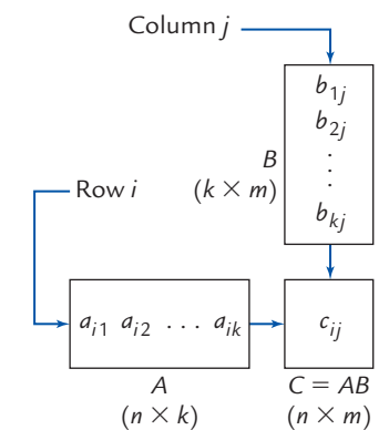
Figure 2 Computing an entry in matrix multiplication.
