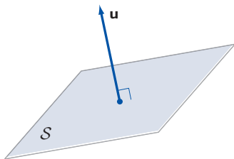
Figure 4 A subspace S and orthogonal vector \mathbf{u} .
