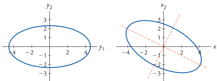
(a) Graph of 2y_1^2 + 7y_2^2 = 40
