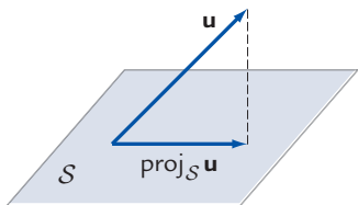
Figure 3 Projection of a vector \mathbf{u} in \mathbb{R}^3 onto a two-dimensional subspace S .
