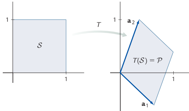
Figure 1 The square S and \mathcal{P} = T(S) , where T(\mathbf{x}) = A\mathbf{x} and A = [\mathbf{a}_1 \ \mathbf{a}_2] .
