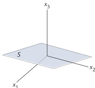
Figure 1 The subspace S in \mathbf{R}^3 .
