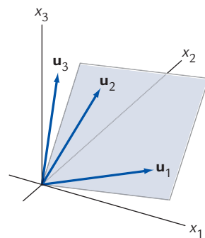
Figure 2 Any three nonzero vectors that do not lie in the same plane forms a basis for \mathbb{R}^3 .
